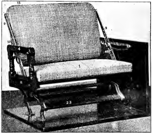
Fig. 3983. SWING-BACK RATTAN-SEAT.
